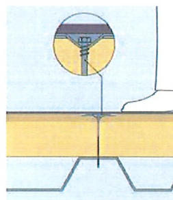
A bonded membrane incorporating HARDROCK® Multi-Fix (DD)
