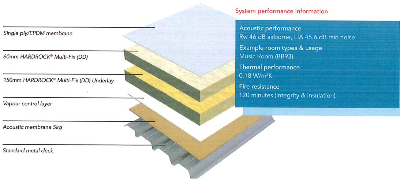
Example 2 - Dual layer system (Partial/fully bonded or mechanically fixed)
